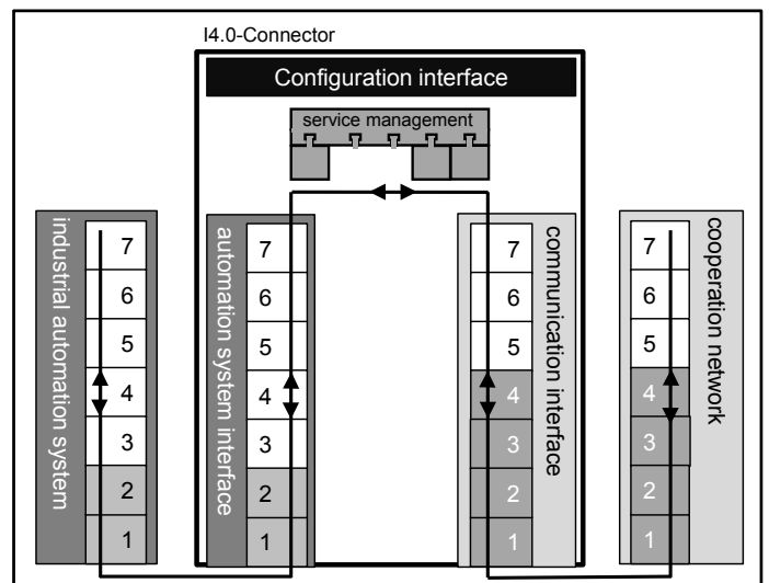
Fig. 2: The connection of two networks with different communication protocols
